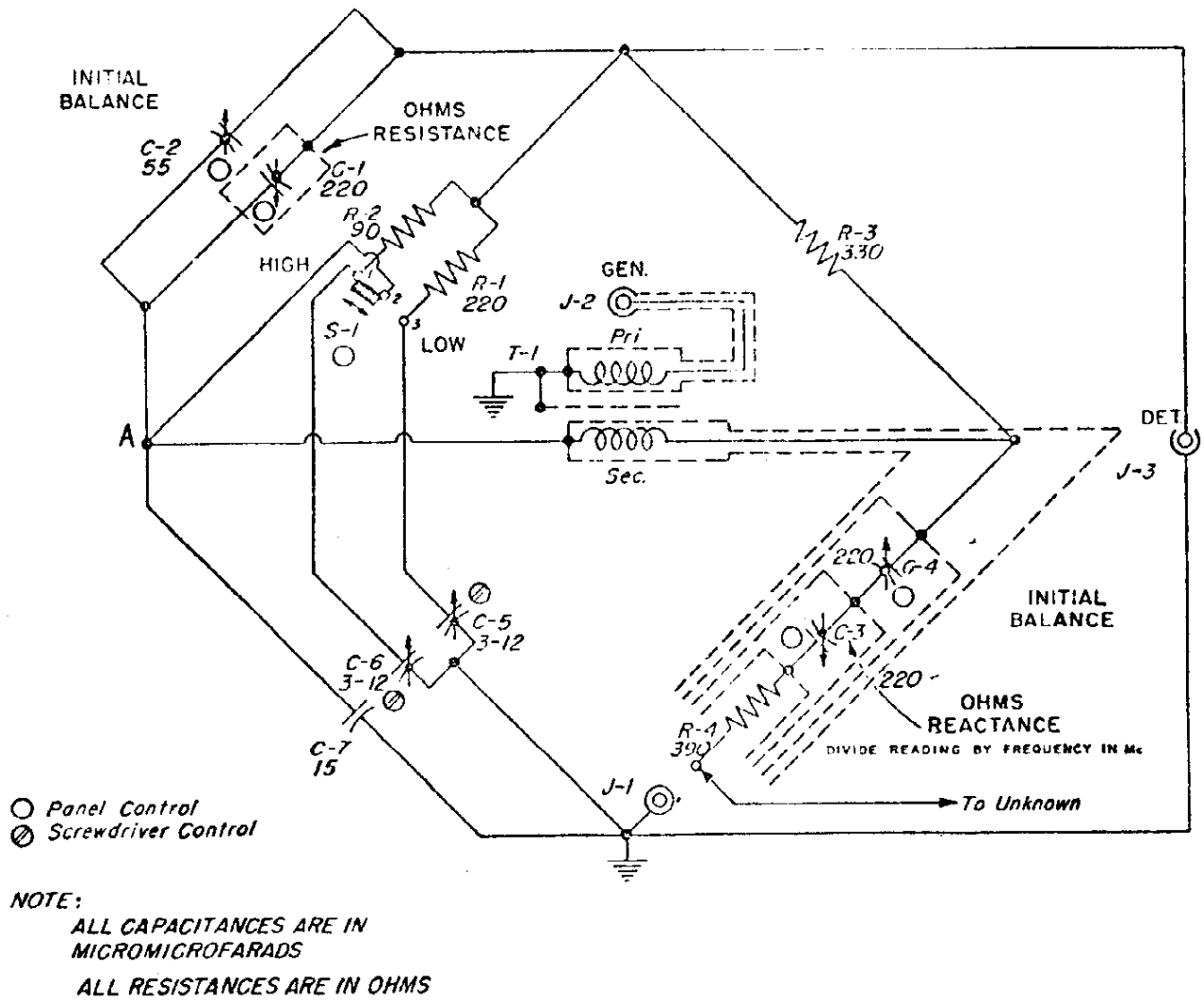
Figure 10. Schematic Diagram of Type 1606-A R-F Bridge.
